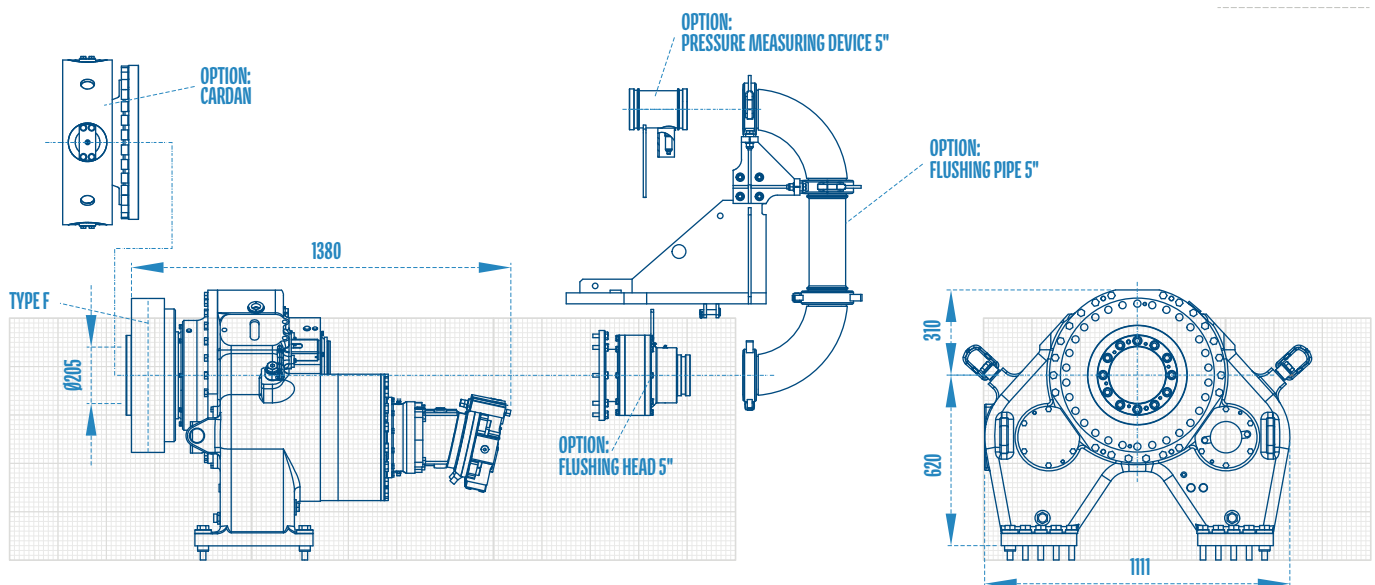
DRILLING ACCESSORIES
